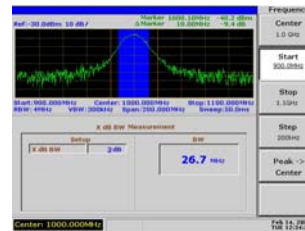
N-dB BW Measurement
